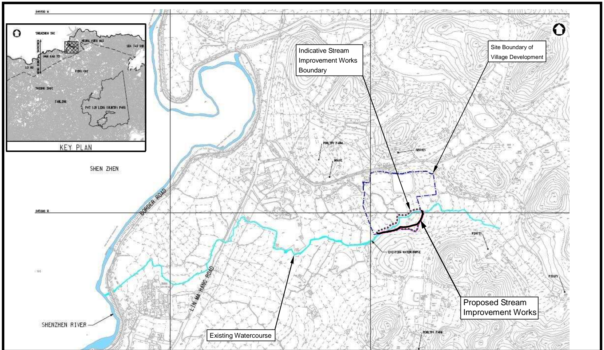
Figure 1 Stream Improvement at Ta Kwu Ling Associated with the Resite of Chuk Yuen Village
